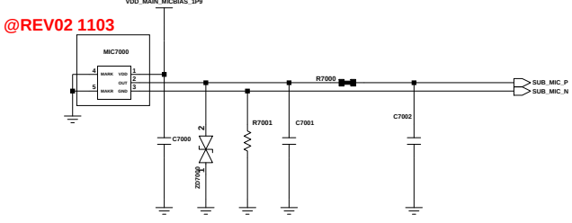
2nd MIC
