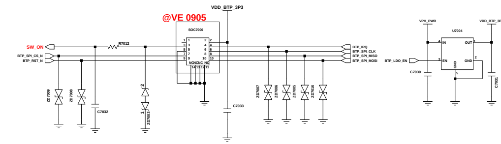
PWR & SIDE FPS
