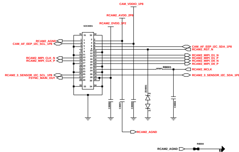
RCAM2 5M UW (30pin) GC5035
