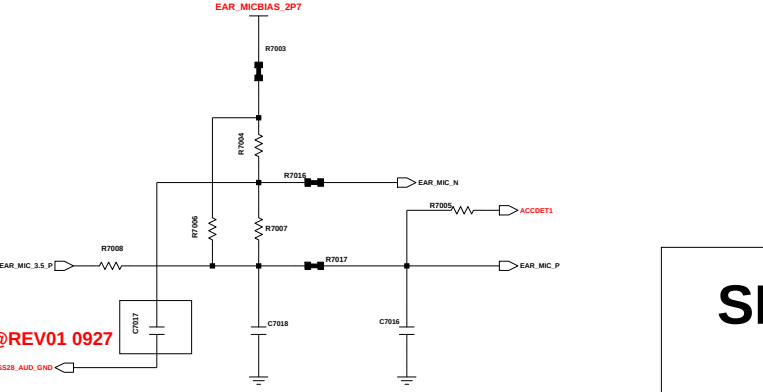
EAR MIC
