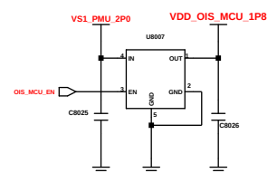
OIS MCH @ STM -> Penesas
