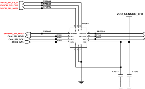
ACC&GYRO SENSOR
