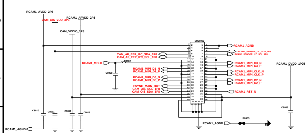
RCAM1_50M(OIS_40PIN)
