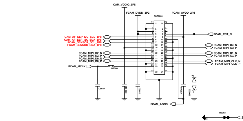
FRONT 13M CAMERA
