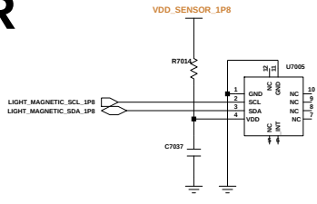
AMBIENT SENSOR
